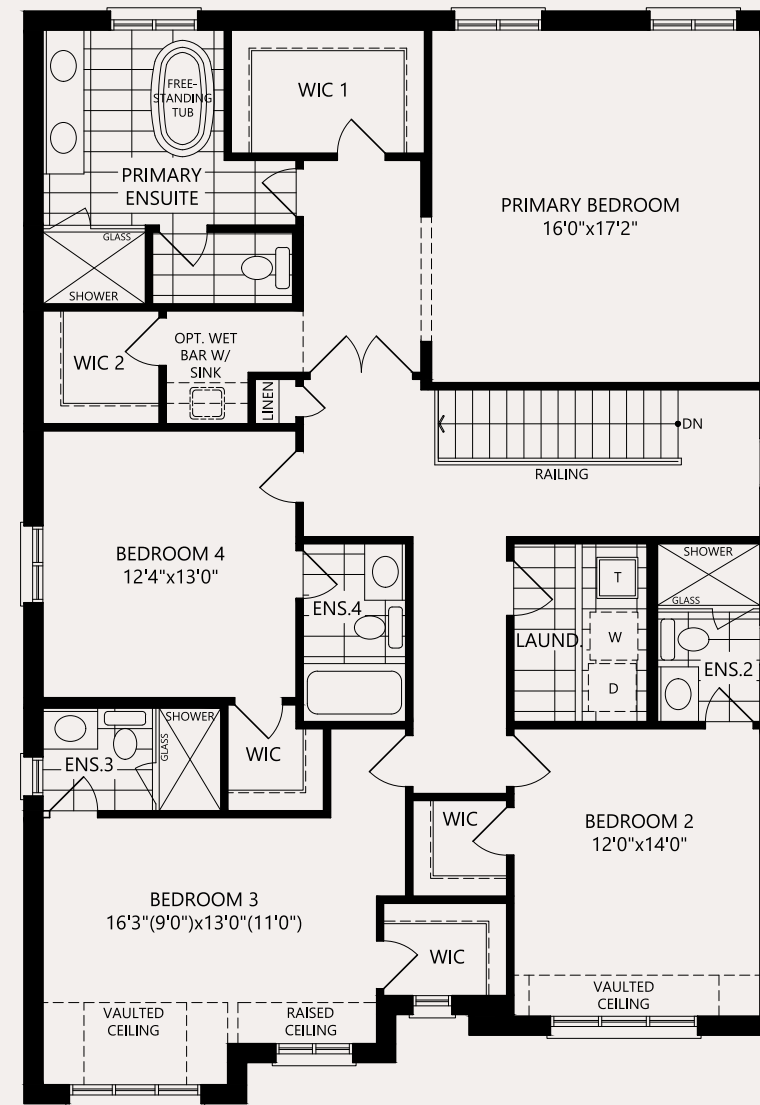
SECOND LEVEL – 4 BEDROOM
