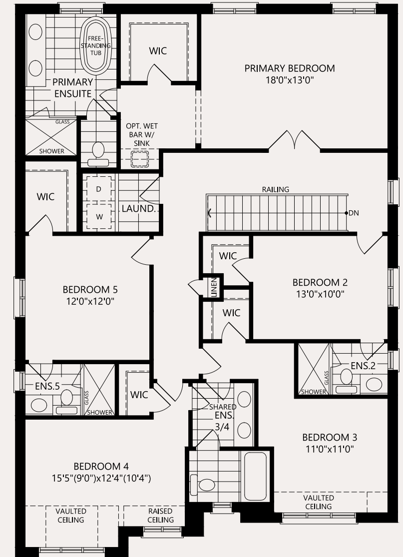
SECOND LEVEL – 5 BEDROOM
