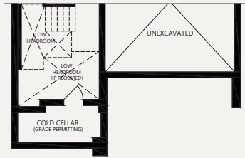
PARTIAL BASEMENT
