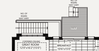
PARTIAL GROUND
