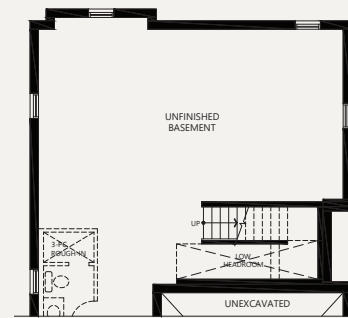
PARTIAL BASEMENT
