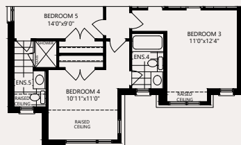
PARTIAL SECOND LEVEL 5 BED + 4 BATH OPTION
