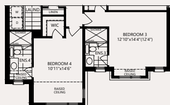
PARTIAL SECOND LEVEL 4 BED + 4 BATH OPTION
