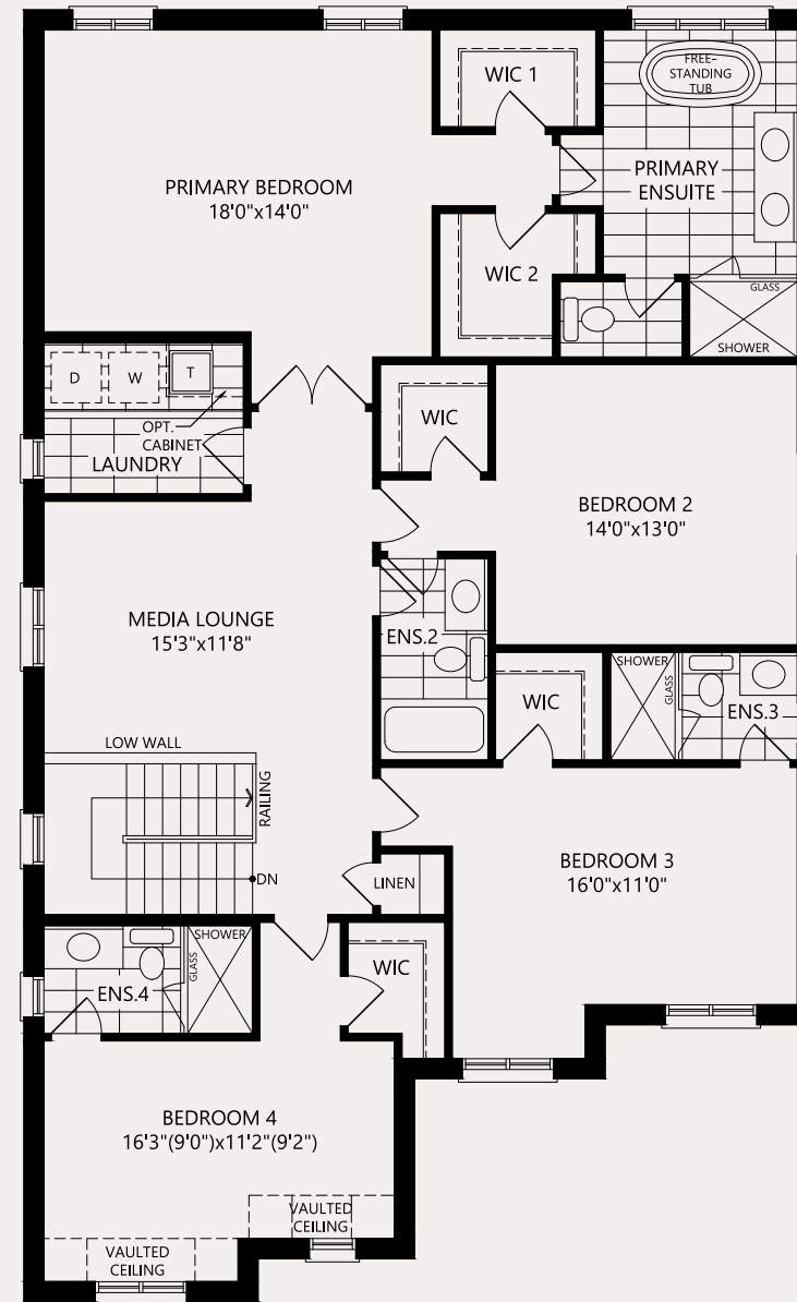
SECOND LEVEL - 4 BEDROOM
