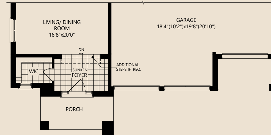
MAIN FLOOR
