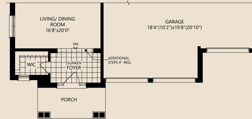
MAIN FLOOR
